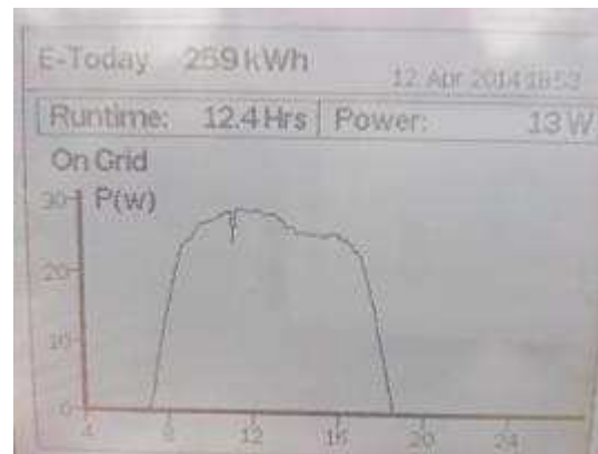
Inverter 2
